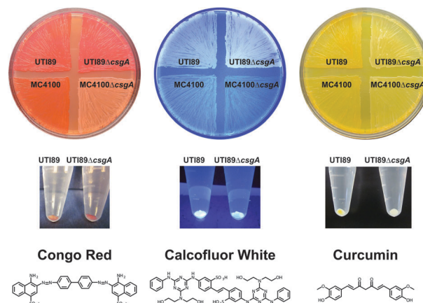
Fig. 1 Dye binding to MC4100 and UTI89 wild-type and curli-mutant strains during growth on YESCA agar plates supplemented with the indicated molecules (top row) and after growth on YESCA agar without compound supplementation via a solution-based pull-down assay (middle row). CR binding is not curli specific in UTI89. Calcofluor-based fluorescence indicates the production of cellulose by UTI89 and UTI89ΔcsgA. Curcumin exhibits curli-specific binding in UTI89 even in the presence of cellulose.
