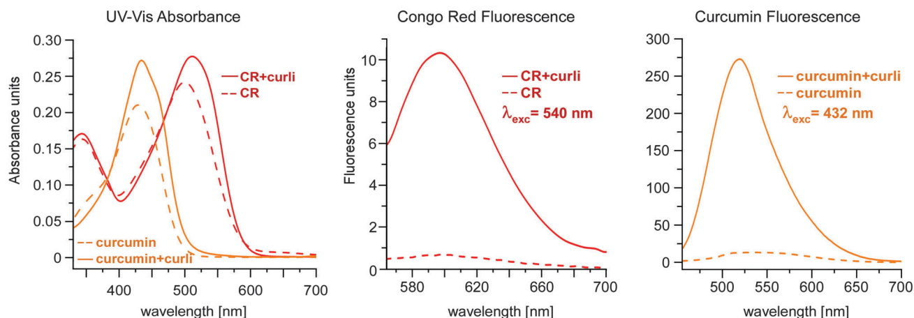
Fig. 2 Binding of curcumin to curli results in a red shift in the absorbance spectrum, similar to the spectral shift observed for Congo red and commonly used to characterize amyloids (left). Like Congo red, curcumin exhibits significantly enhanced fluorescence when bound to curli (middle and right).
